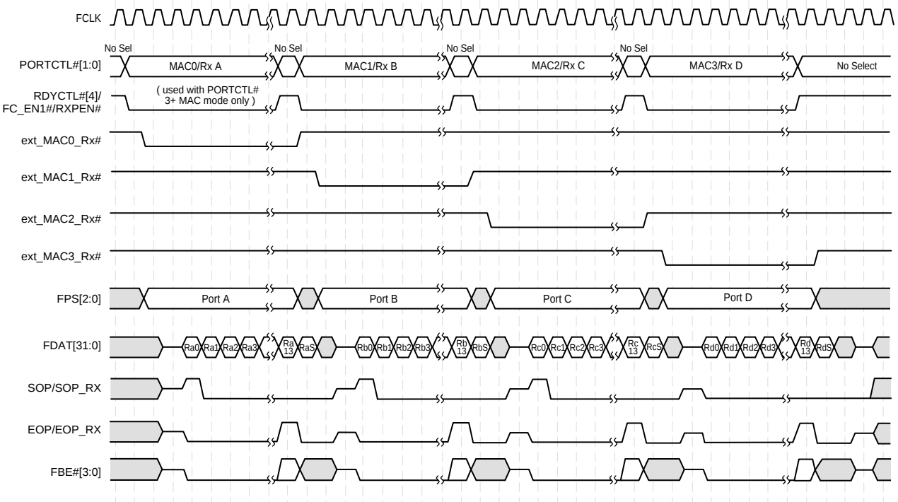
Figure 41. 32-Bit Unidirectional IX Bus Timing - Consecutive Receives, EOP on 14th Data Return with Status
