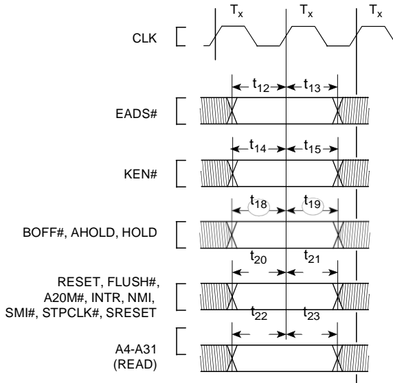
Figure 10. Input Setup and Hold Timing
