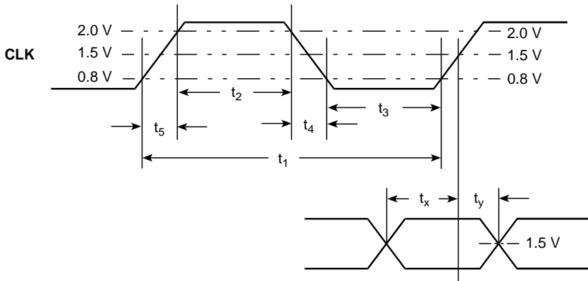
Figure 9. CLK Waveform
