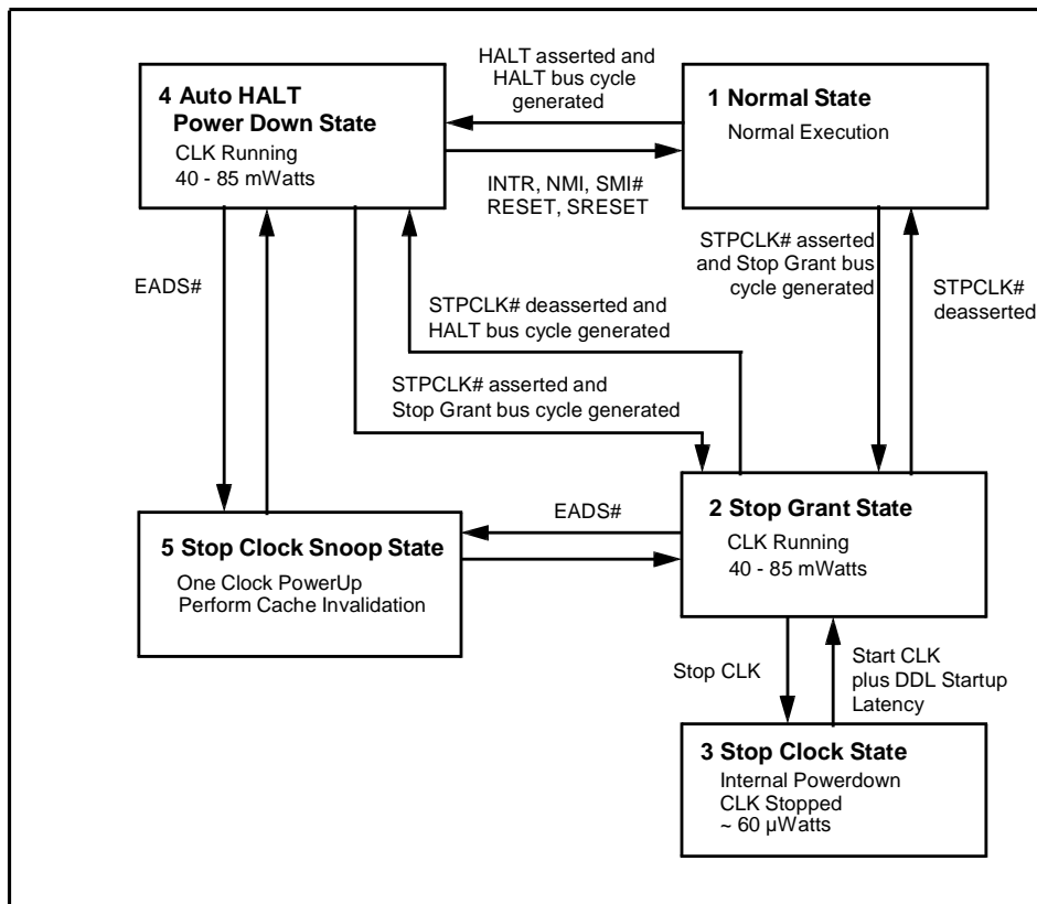
Figure 4. Stop Clock State Diagram with Typical Power Consumption Values
