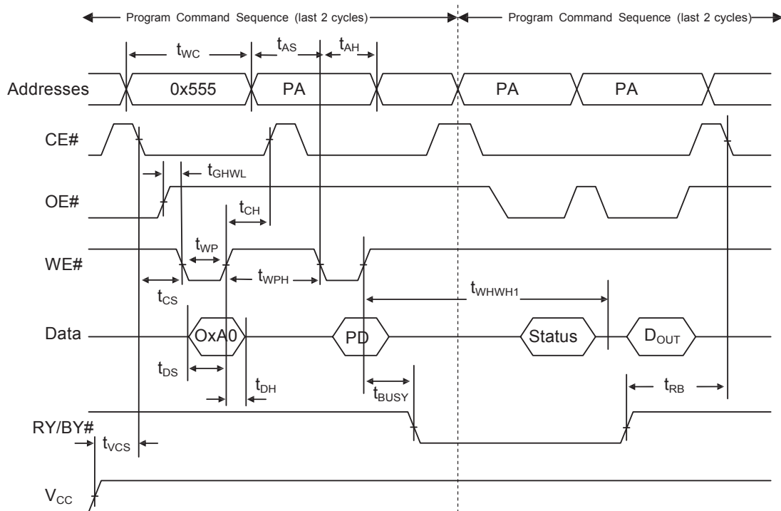
Figure 5. Program Operation Timings
