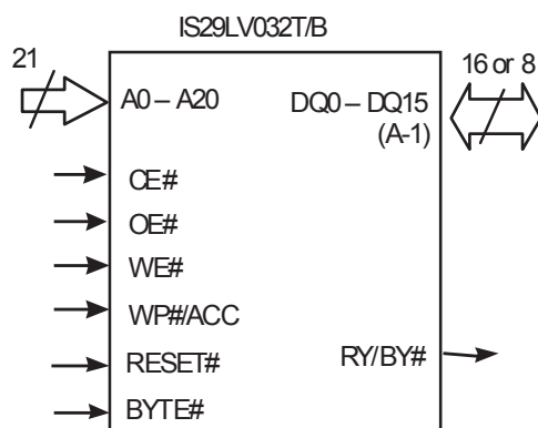
LOGIC DIAGRAM
