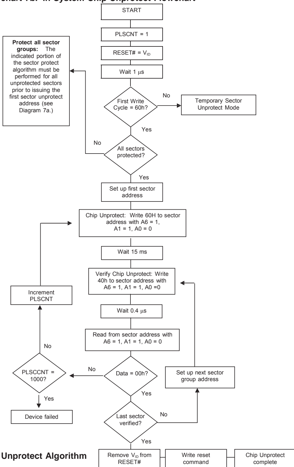
Flowchart 7b. In-System Chip Unprotect Flowchart
