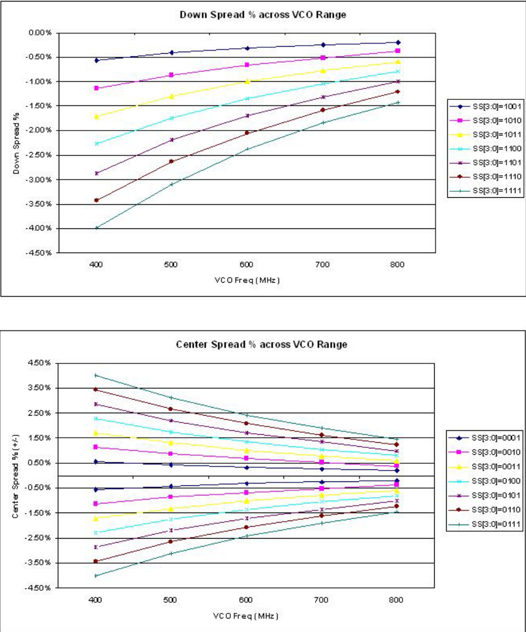
Figure 5. Center Spread % across VCO Range with 16 MHz Reference
