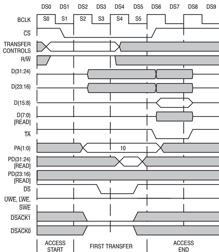
Figure 45. 8-Bit '040 READ From 16-Bit Peripheral Example (PA1,PA0=10)
