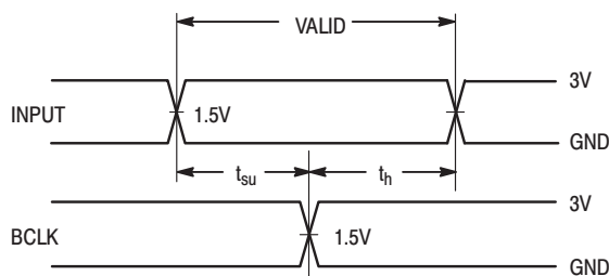
Figure 11. Setup/Hold Times
