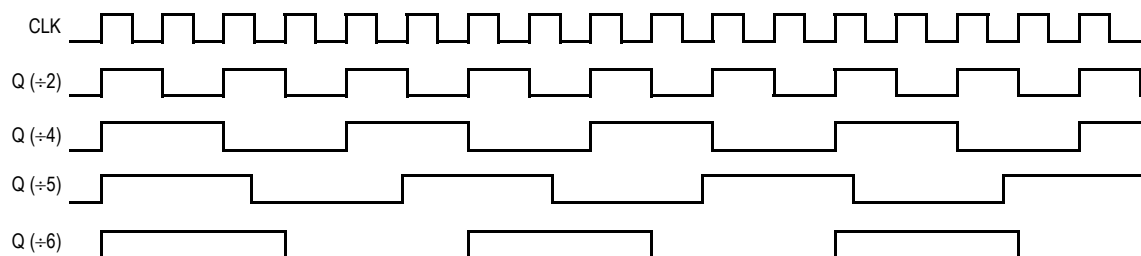
Figure 3. Timing Diagram
