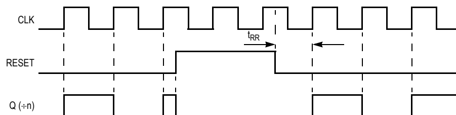
Figure 4. Timing Diagram
