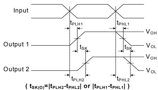
Figure 3. Output Skew
