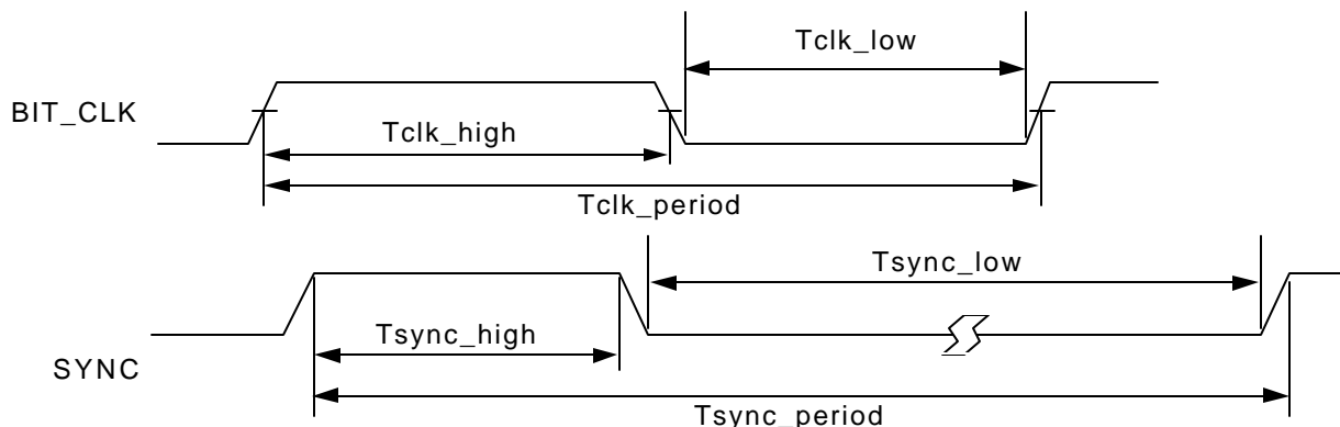
Figure 4. Clocks Timing
