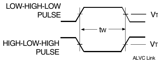
Pulse Width
