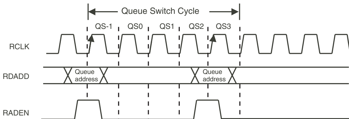
Figure 10. Read Port Switching Queues Signal Sequence
