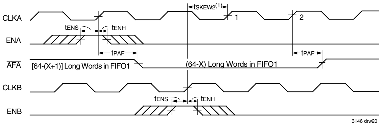
Figure 19. Timing for AEA when FIFO2 is Almost-Empty
