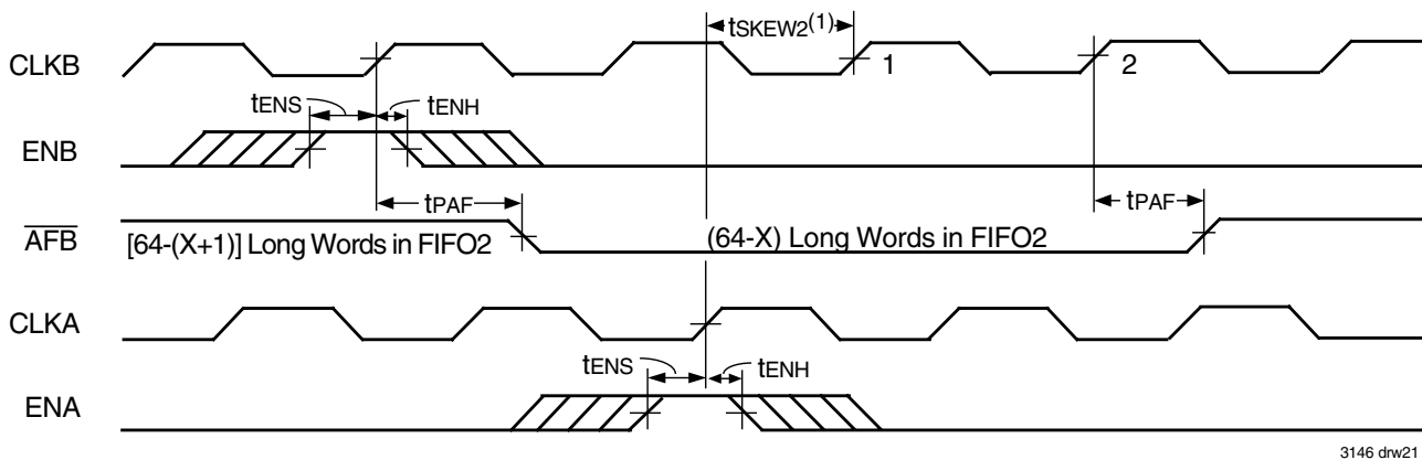
Figure 20. Timing for AFA when FIFO1 is Almost-Full
