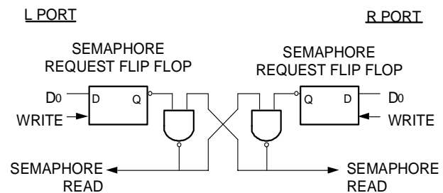
Figure 4. IDT70P27 Semaphore Logic 5694 drw 18
