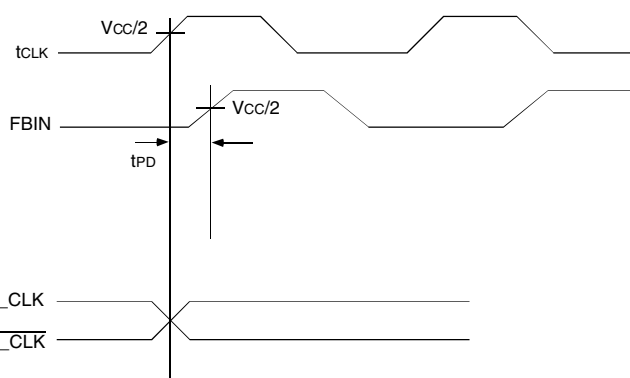
Prop Delay
