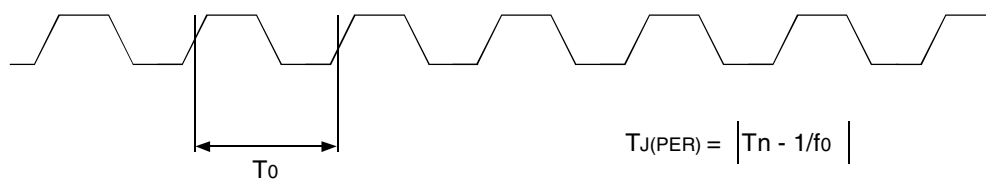
Period Jitter
