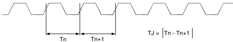
Cycle-to-Cycle Jitter
