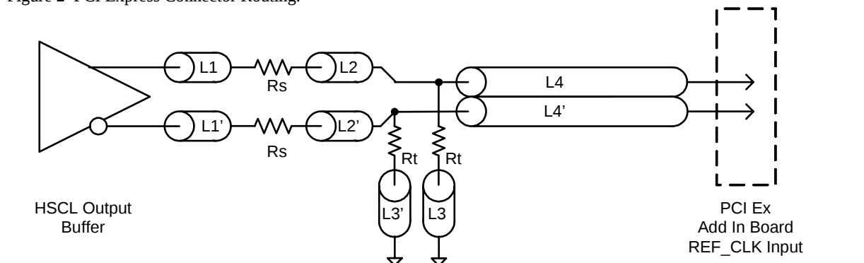
Figure 2 PCI Express Connector Routing.
