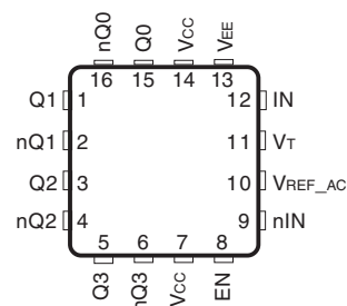
ICS889831 16-Lead VFQFN 3mm x 3mm x 0.95 package body K Package Top View
