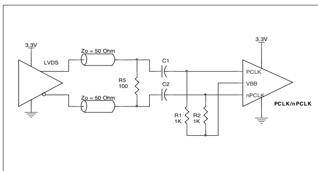
FIGURE 3F. HiPerClockS PCLK/nPCLK INPUT DRIVEN BY A 3.3V LVDS DRIVER
