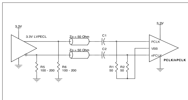
FIGURE 3D. HiPerClockS PCLK/nPCLK INPUT DRIVEN BY A 3.3V LVPECL DRIVER WITH AC COUPLE
