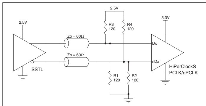
FIGURE 2B. HiPerClockS D/nD INPUT DRIVEN BY AN SSTL DRIVER
