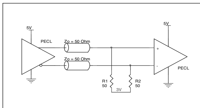
FIGURE 4A. STANDARD 5V LVPECL OUTPUT TERMINATION
