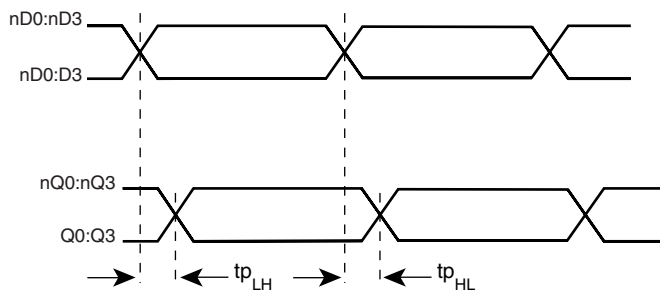
PROPAGATION DELAY
