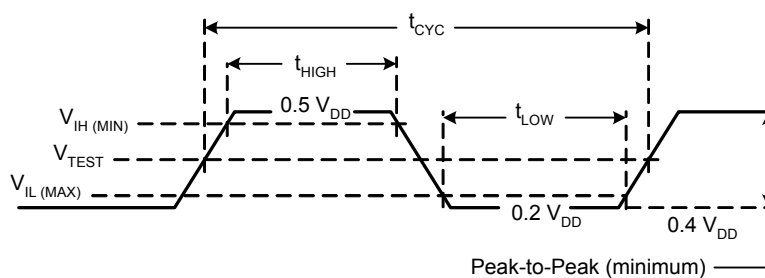
Figure 4. Clock Waveform
