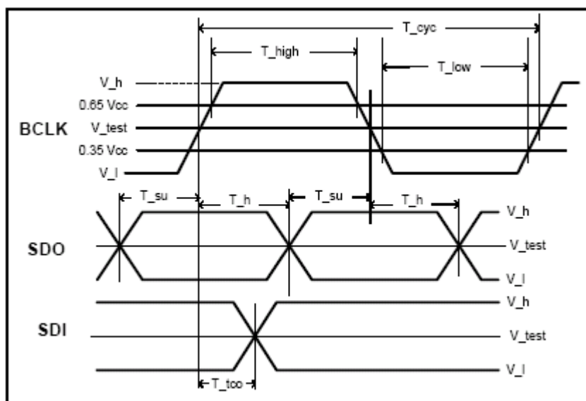
Figure 14. HD Audio Bus Timing
