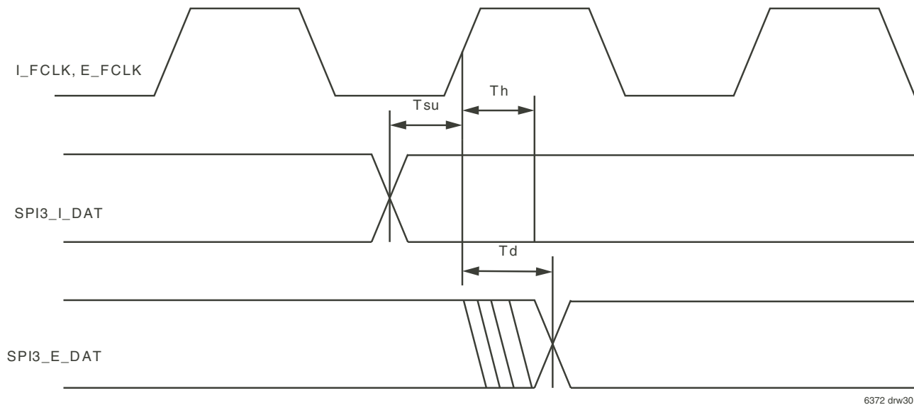
Figure 34. SPI-3 I/O timing diagram
