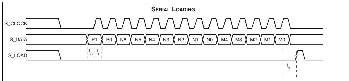
Figure 1. Serial Load Operation
