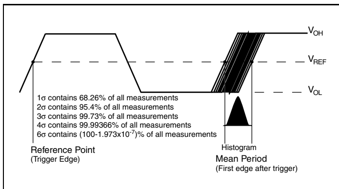
Period Jitter, RMS
