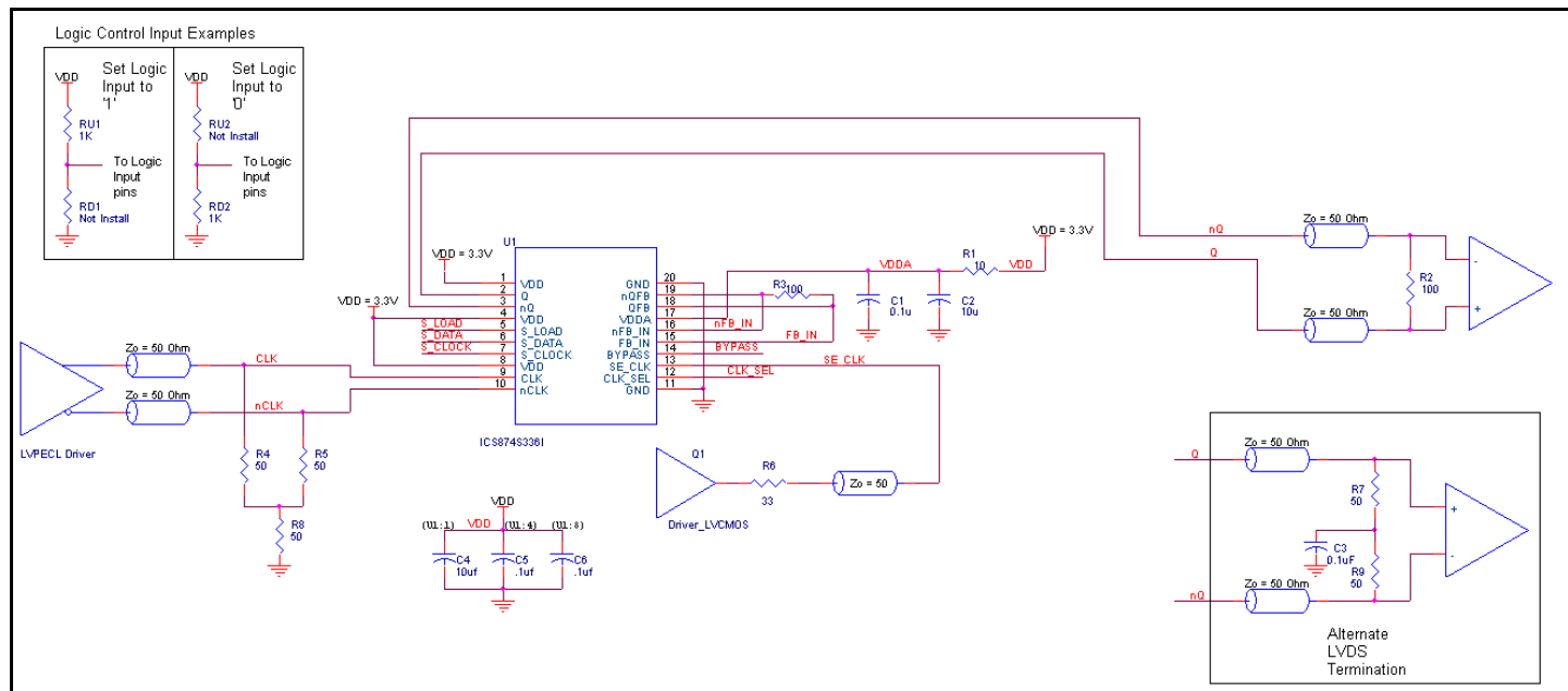
Figure 6. ICS874S336 Schematic Example
