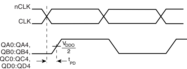
PROPAGATION DELAY
