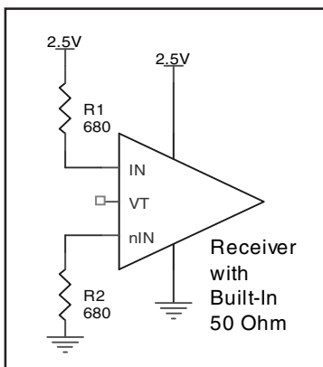
FIGURE 3. UNUSED INPUT HANDLING
