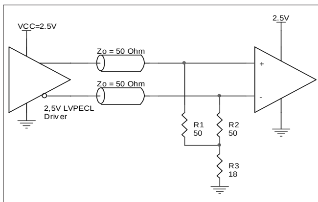
FIGURE 1B. 2.5V LVPECL DRIVER TERMINATION EXAMPLE
