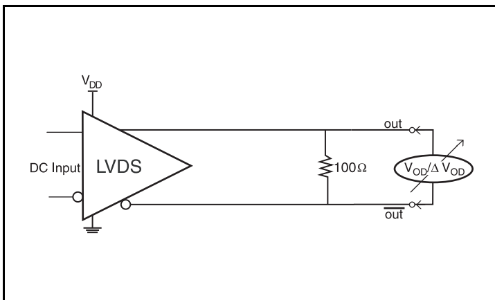
Differential Output Duty Cycle/Pulse Width/Period
