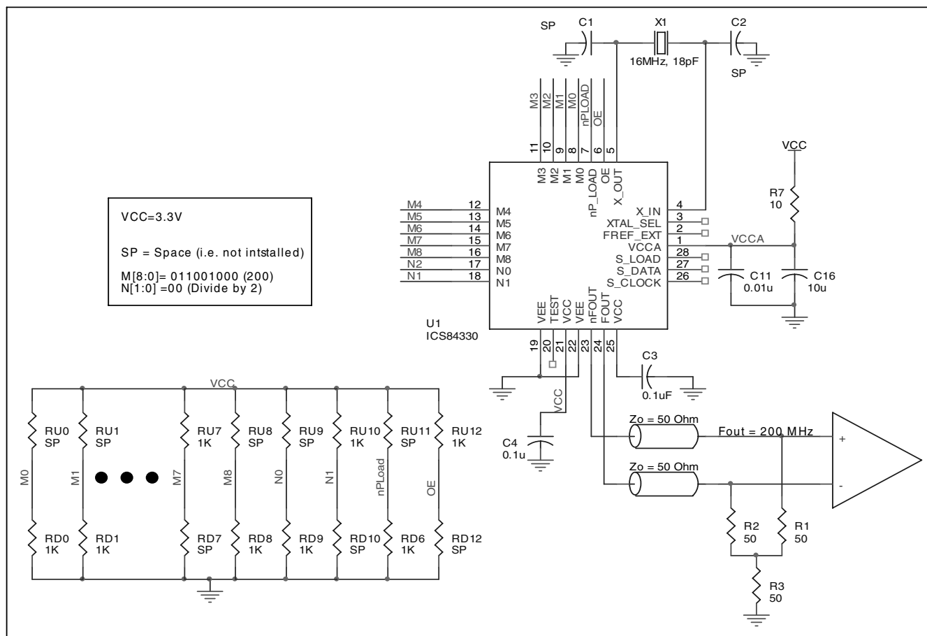
FIGURE 7A. SCHEMATIC OF RECOMMENDED LAYOUT
