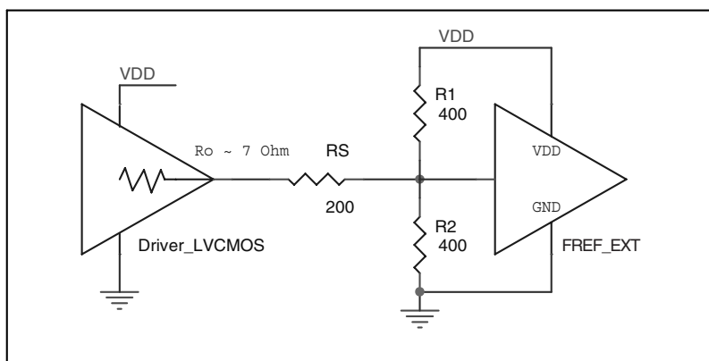
FIGURE 4C. EDGE RATE REDUCTION BY INCREASING THE RESISTOR VALUE
