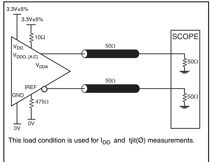
3.3V Core/3.3V HCSL Output Load Test Circuit
