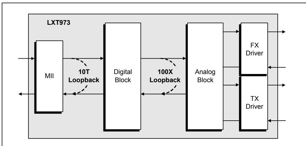
Figure 4 Loopback Paths
