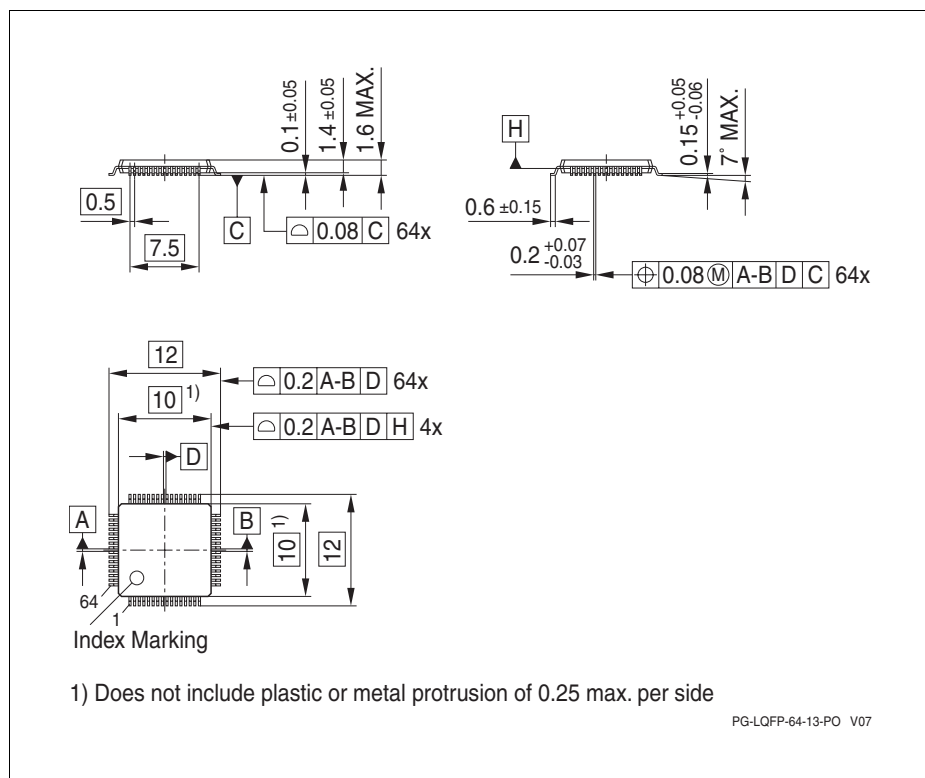
Figure 28 PG-LQFP-64-13 (Plastic Green Thin Quad Flat Package)
