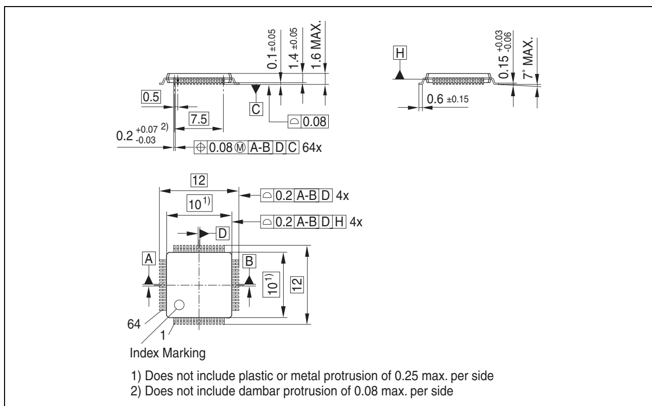
Figure 19 PG-TQFP-64-8 (Plastic Thin Quad Flat Package), valid for the -4F/8F derivatives
