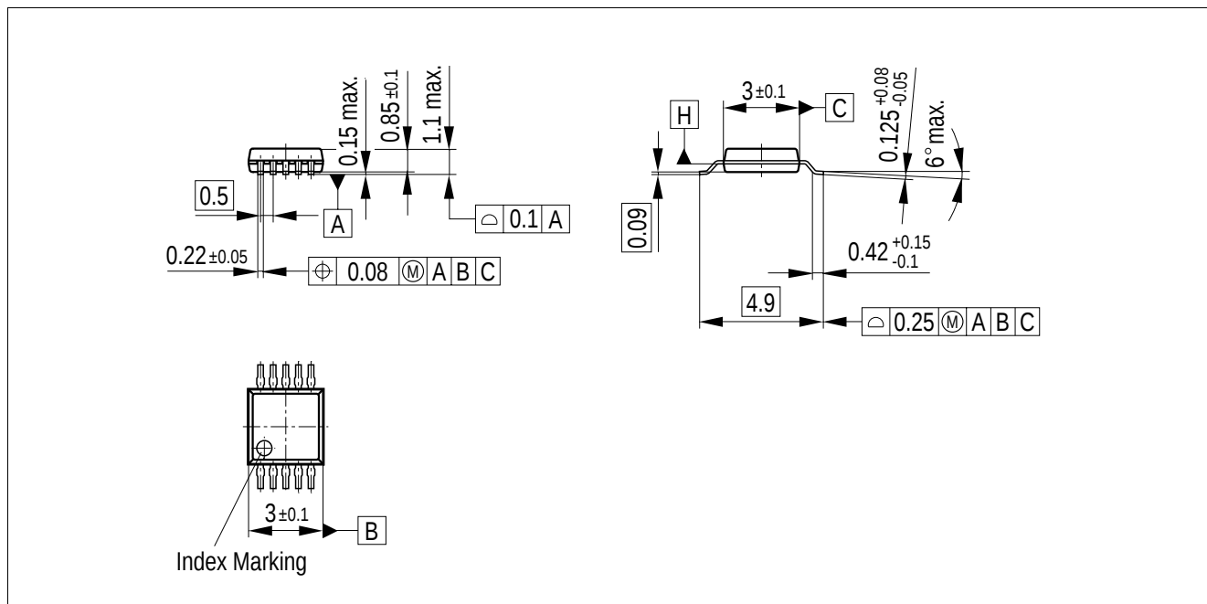
Figure 8 PG-TSSOP-10
