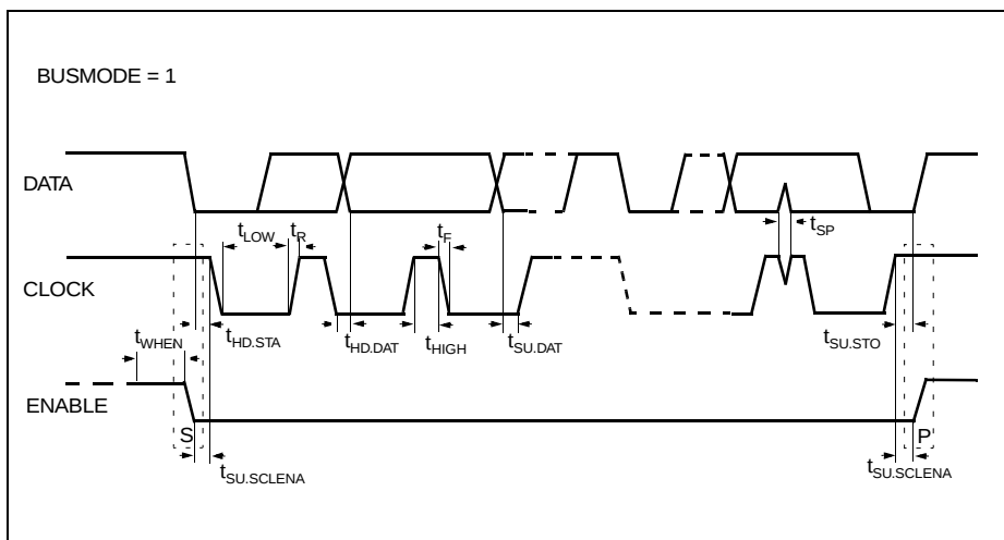
Figure 8 3-Wire Bus
