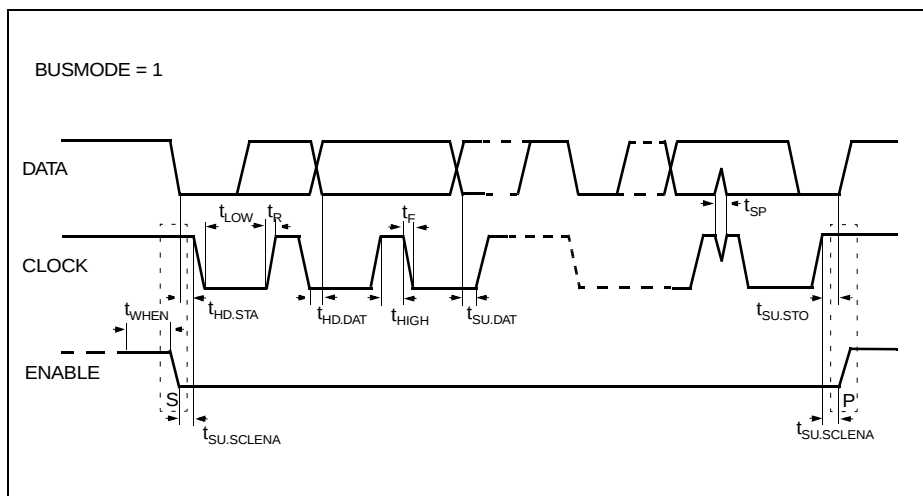
Figure 8 3-Wire Bus
