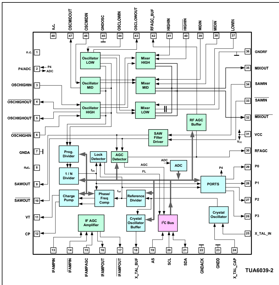
Figure 4 Functional Block Diagram of TUA 6039-2
