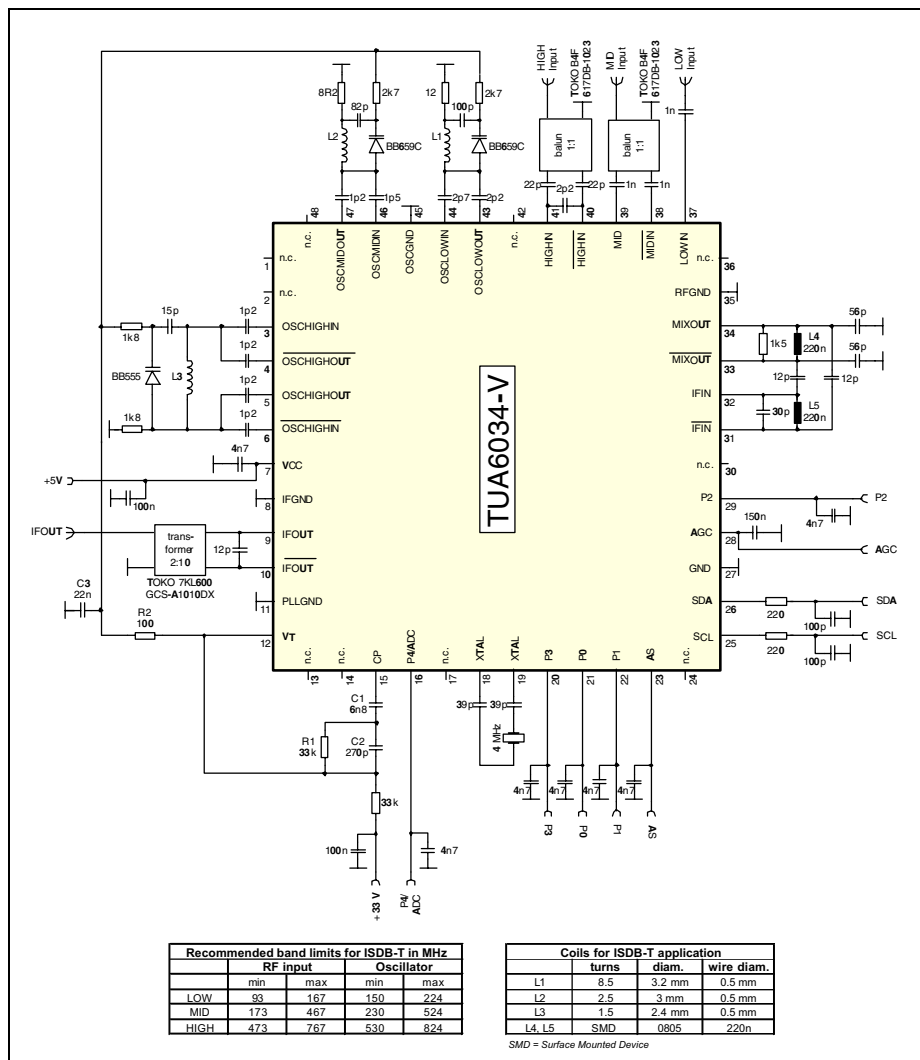
Application Circuit TUA6034-V for ISDB-T
