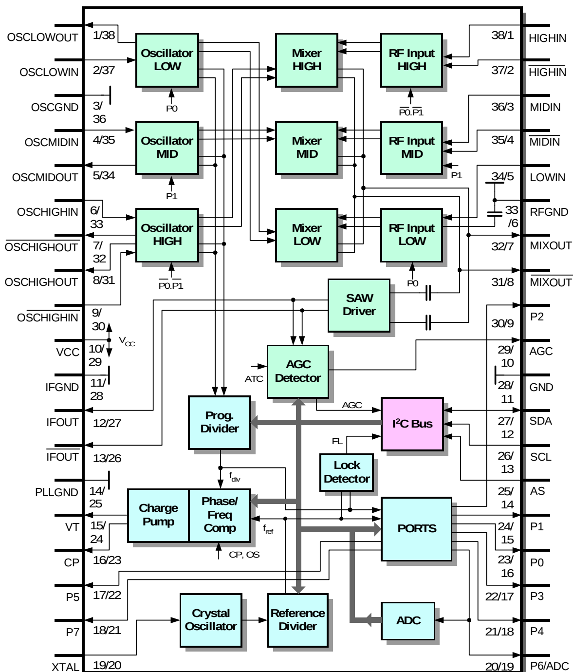
Figure 3-3 Block Diagram
