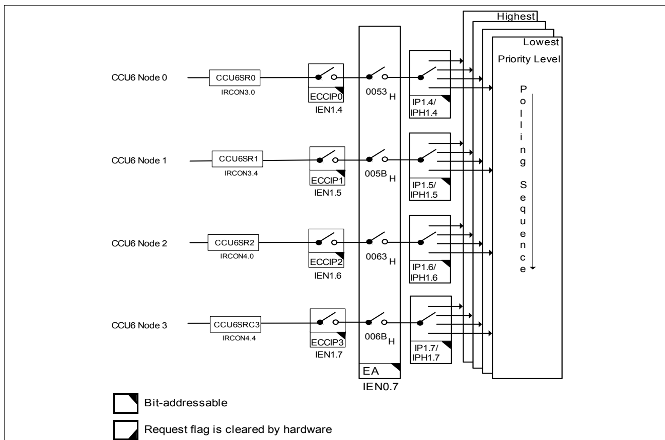
Figure 18 Interrupt Request Sources (Part 5)
