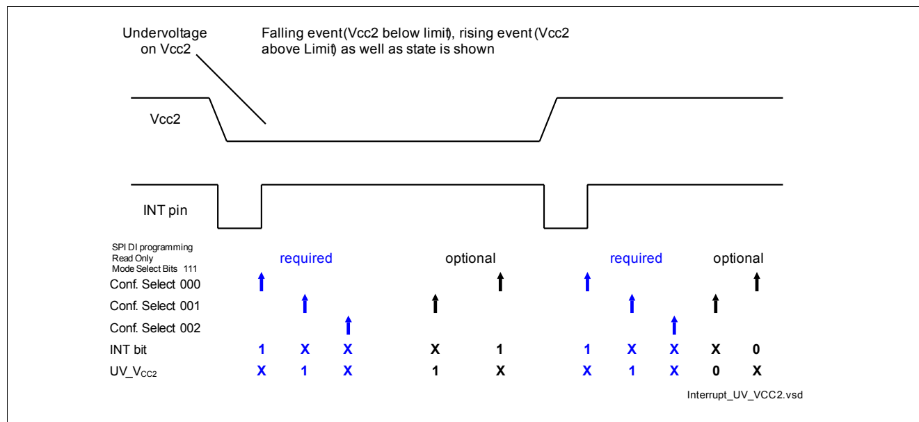
Figure 28 Interrupt V CC2 under-voltage.
