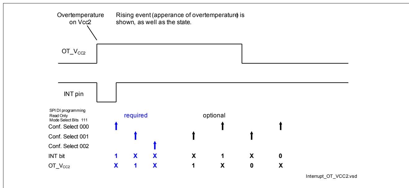
Figure 29 Interrupt Vcc2 Over Temperature.
