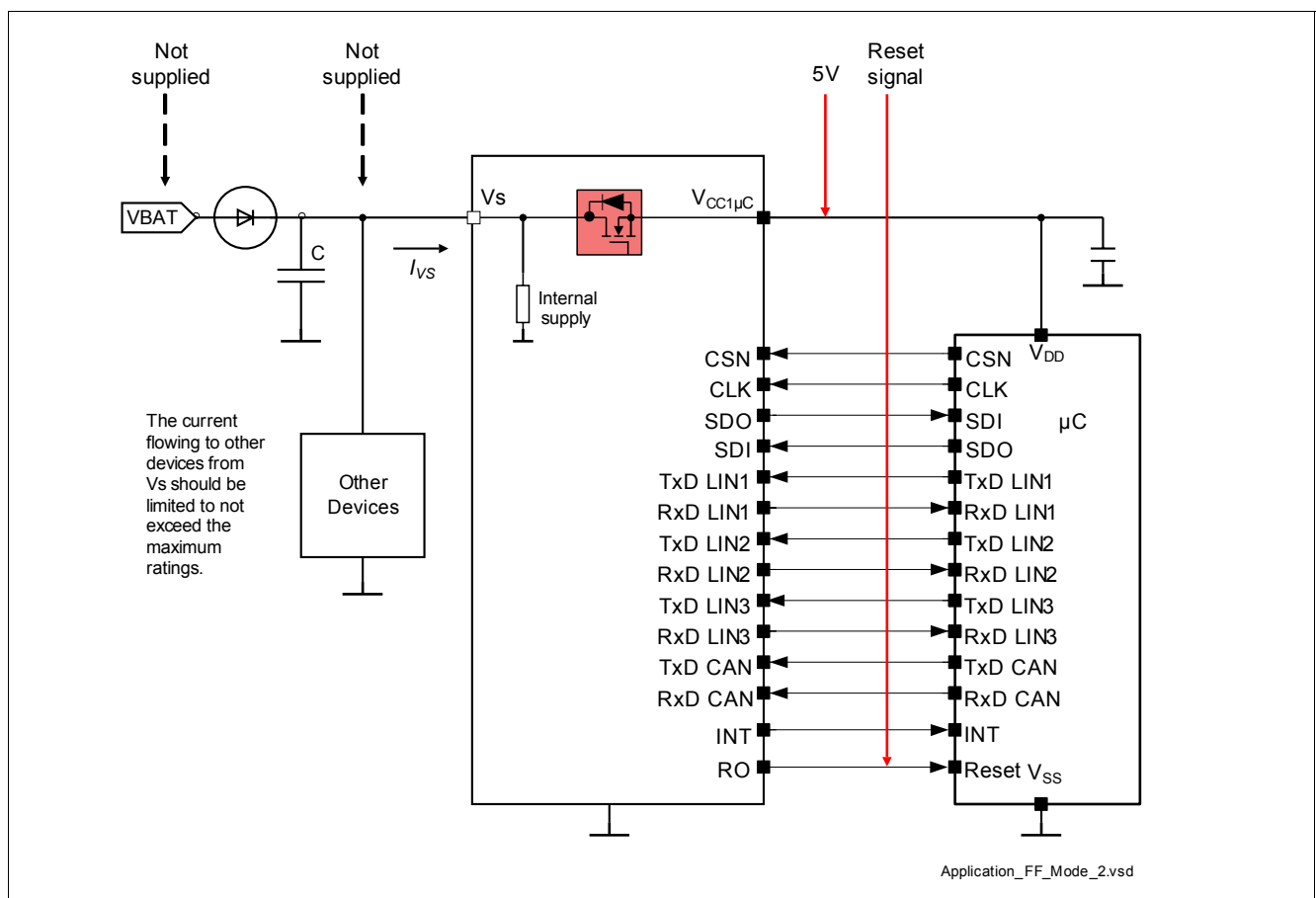
Figure 40 Application Hint for Factor Flash Mode
