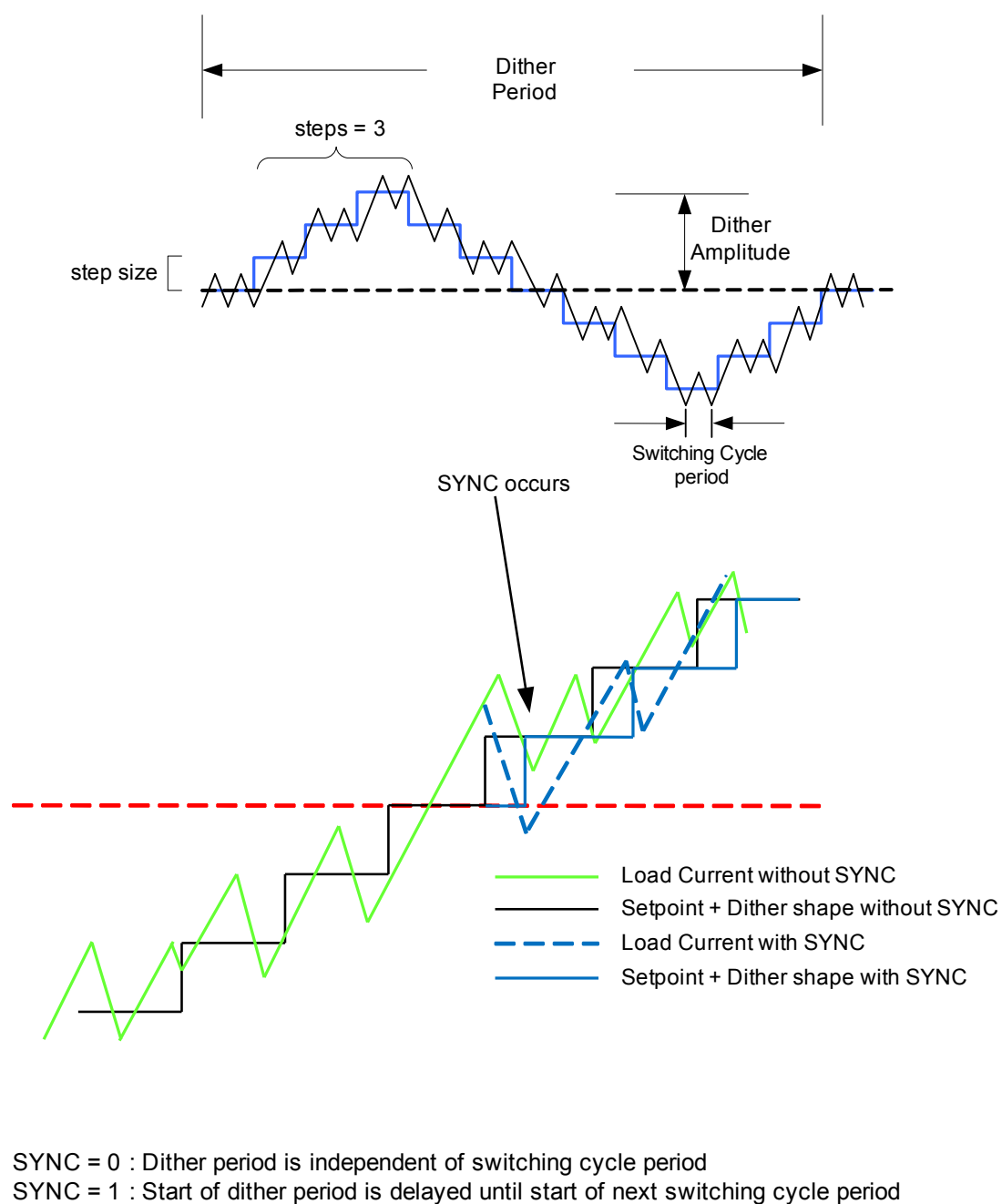
Figure 9 Dither Waveform
