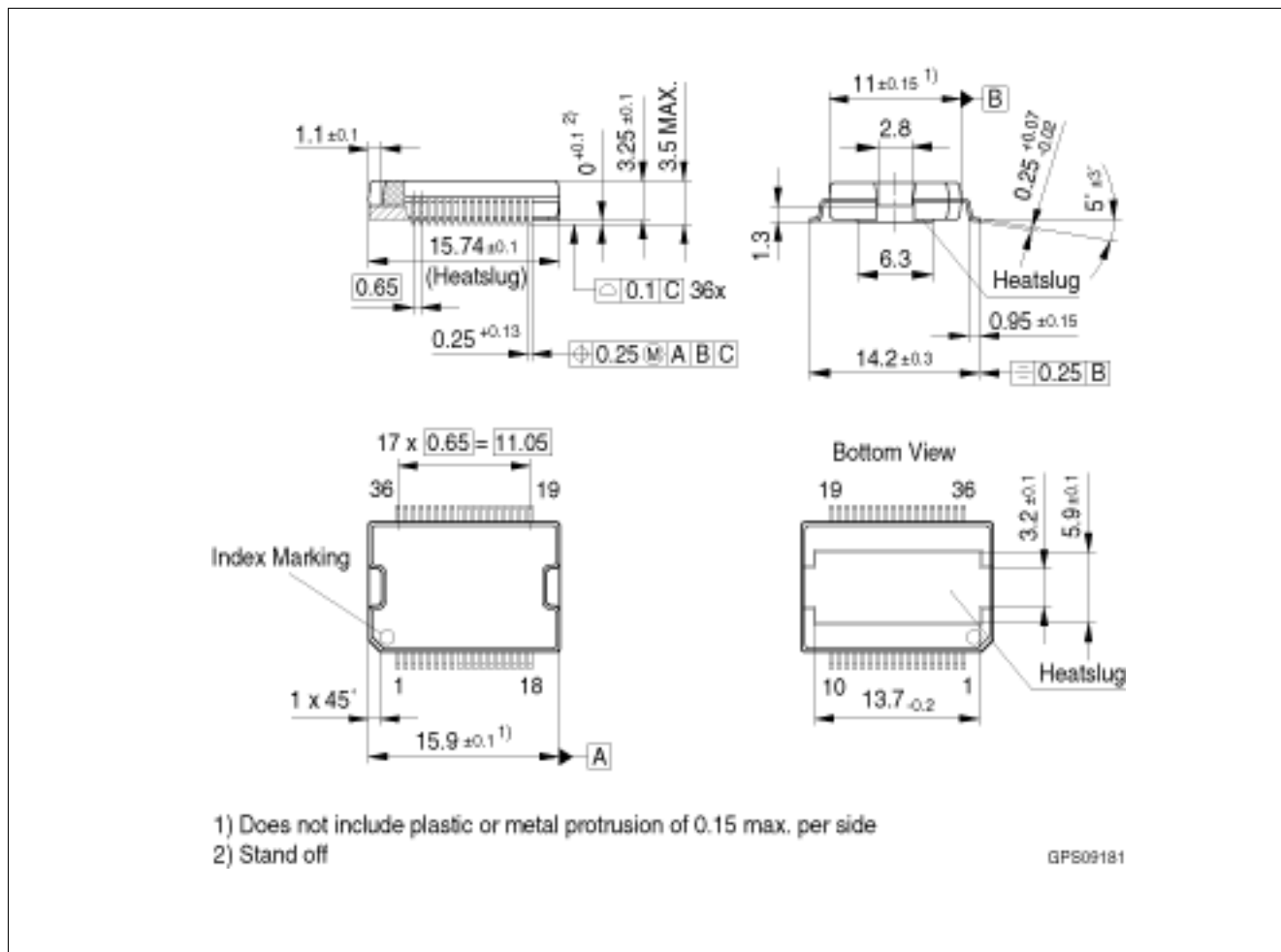
Figure 39 PG-DSO-36
