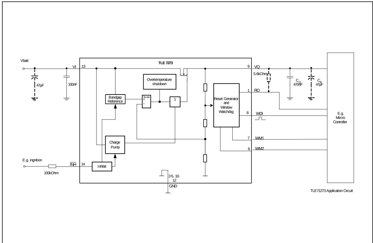
Figure 4 Application Diagram
