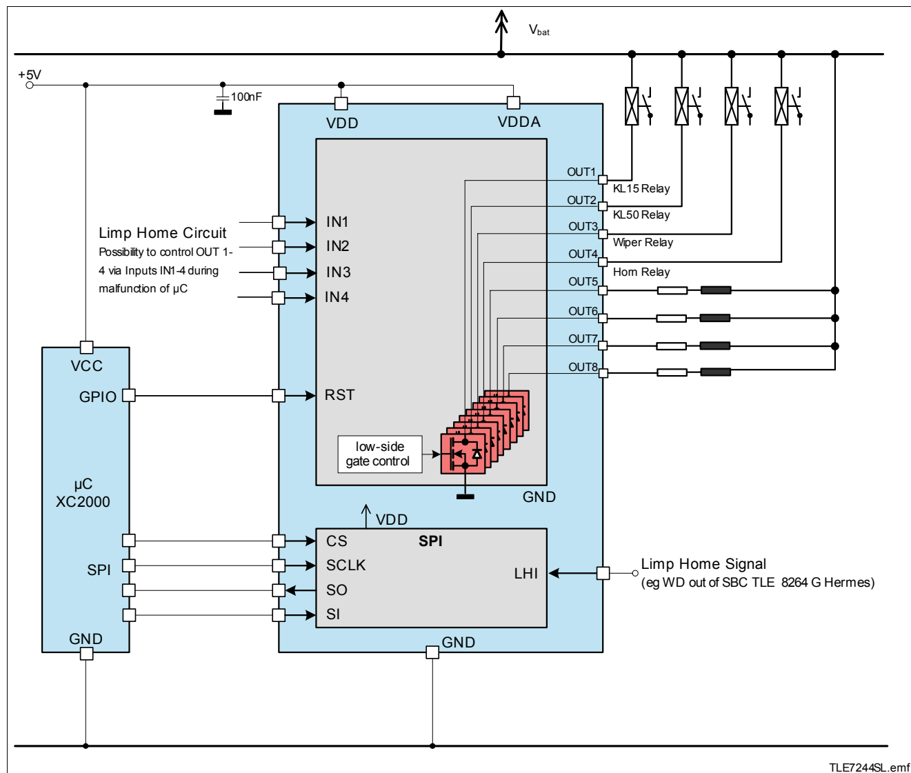
Figure 13 Application Diagram
