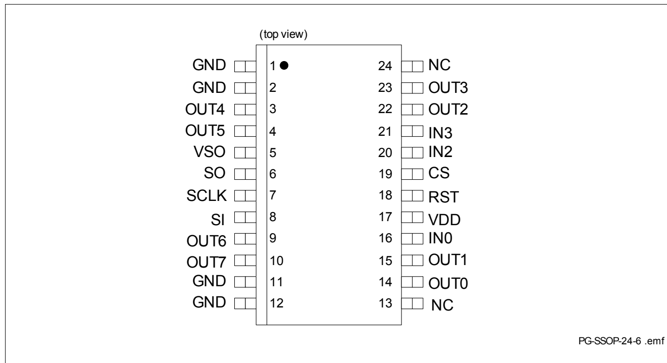
Figure 3 Pin Configuration
