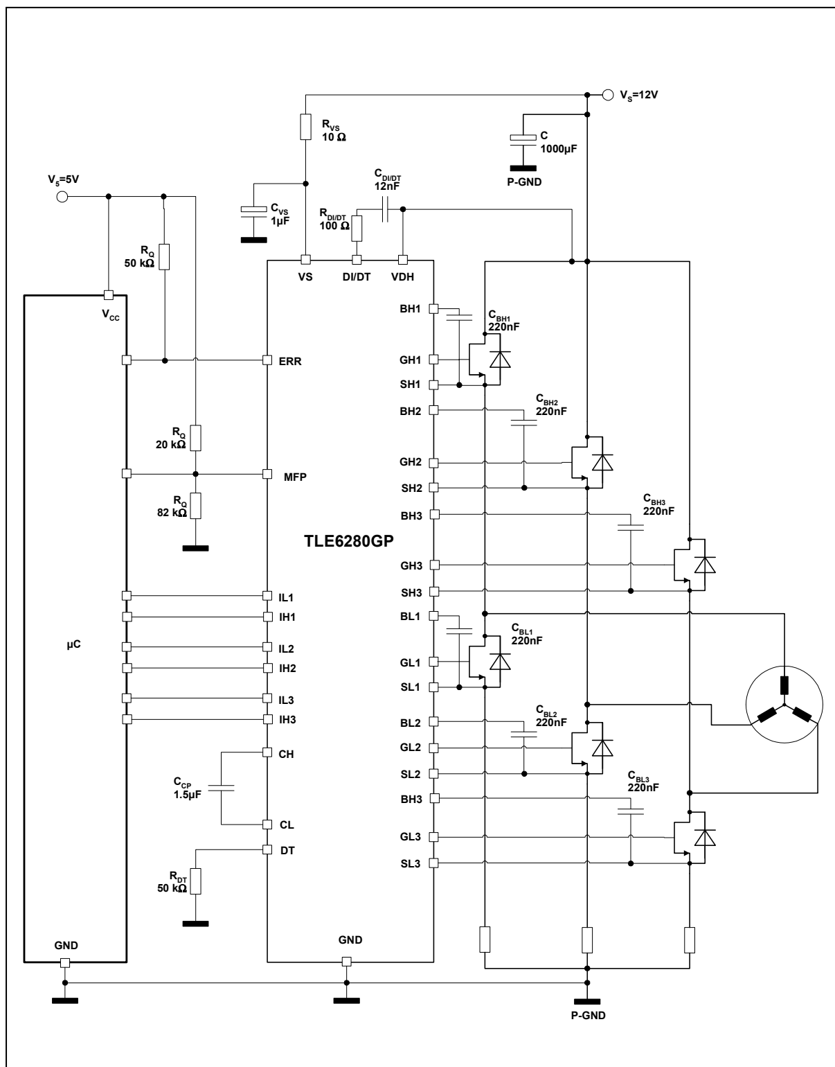
Fig. 1 : Application circuit
