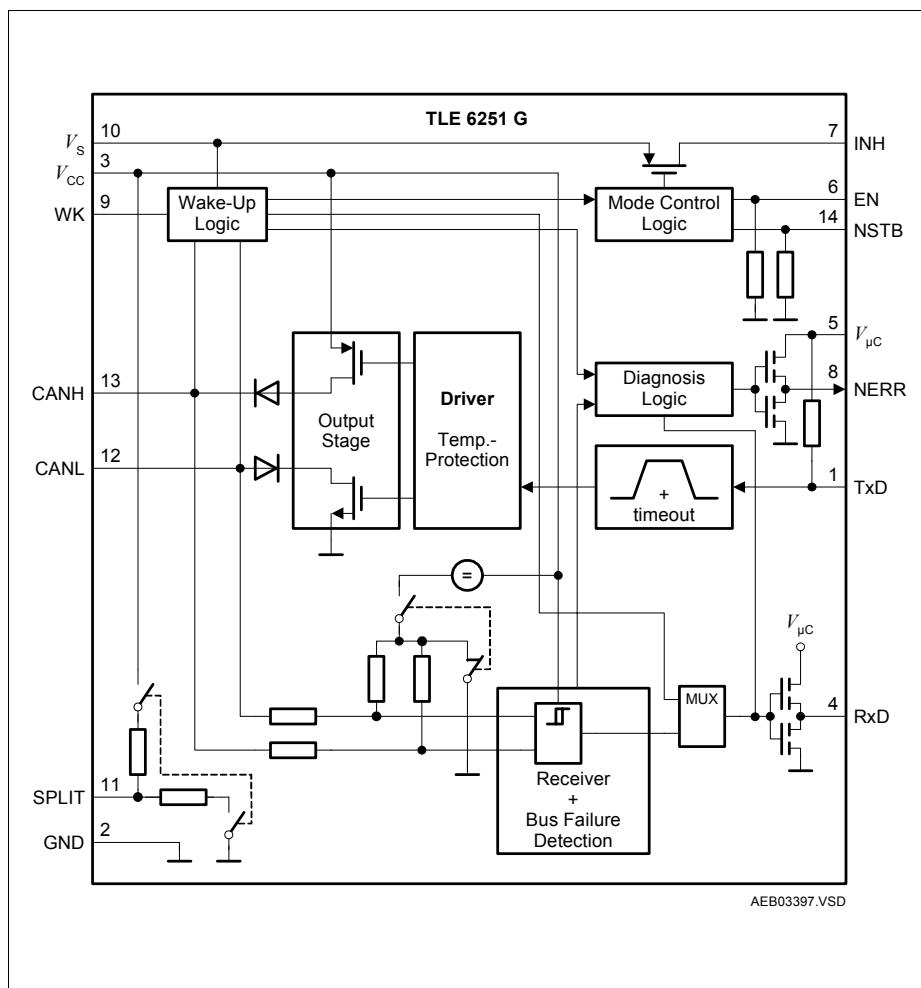
Figure 2 Block Diagram
