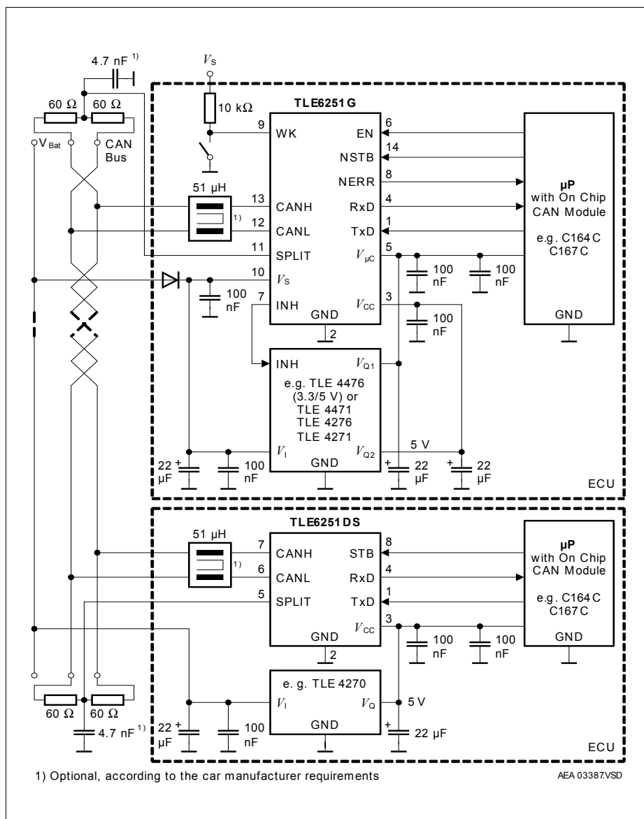
Figure 10 Application Circuit
