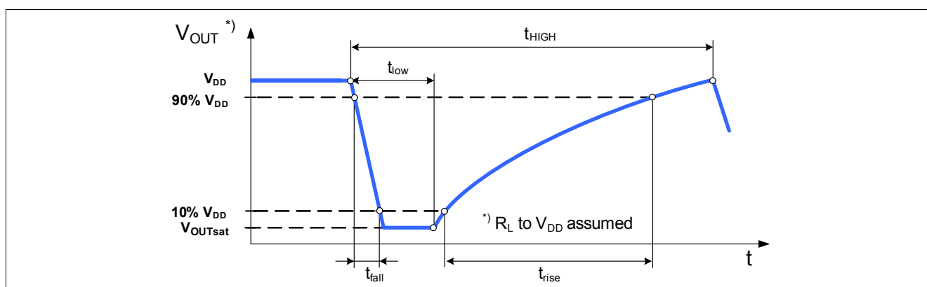
Figure 5-1 Output Characteristic
