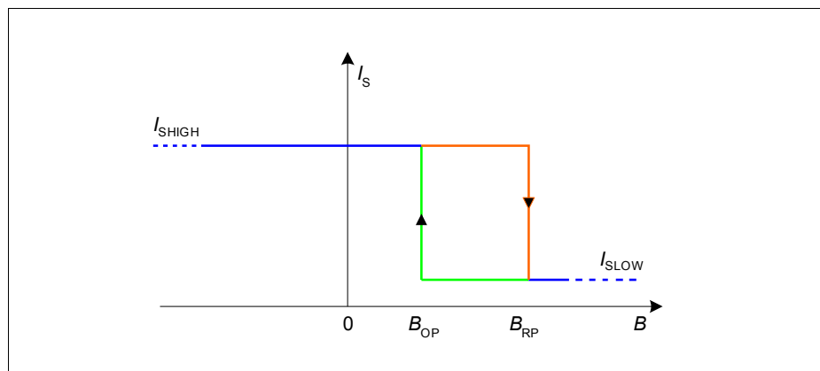
Figure 4 Output Signal
