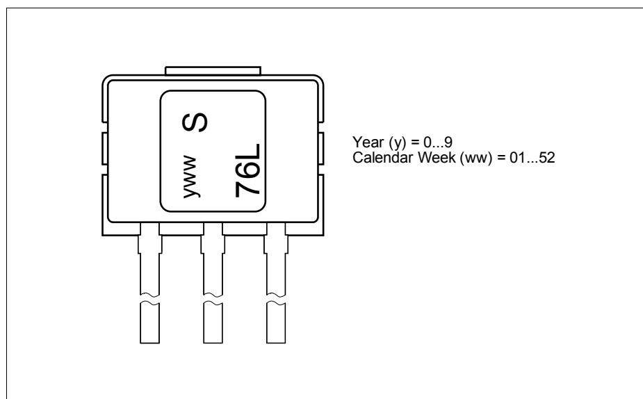
Figure 7 Marking TLE4976L
