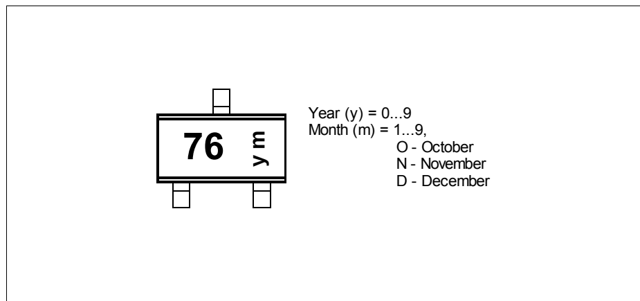
Figure 6 Marking TLE4976-1H
