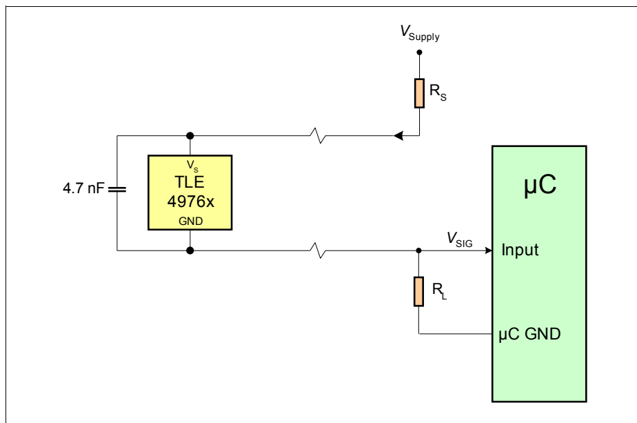
Figure 5 Application Circuit
