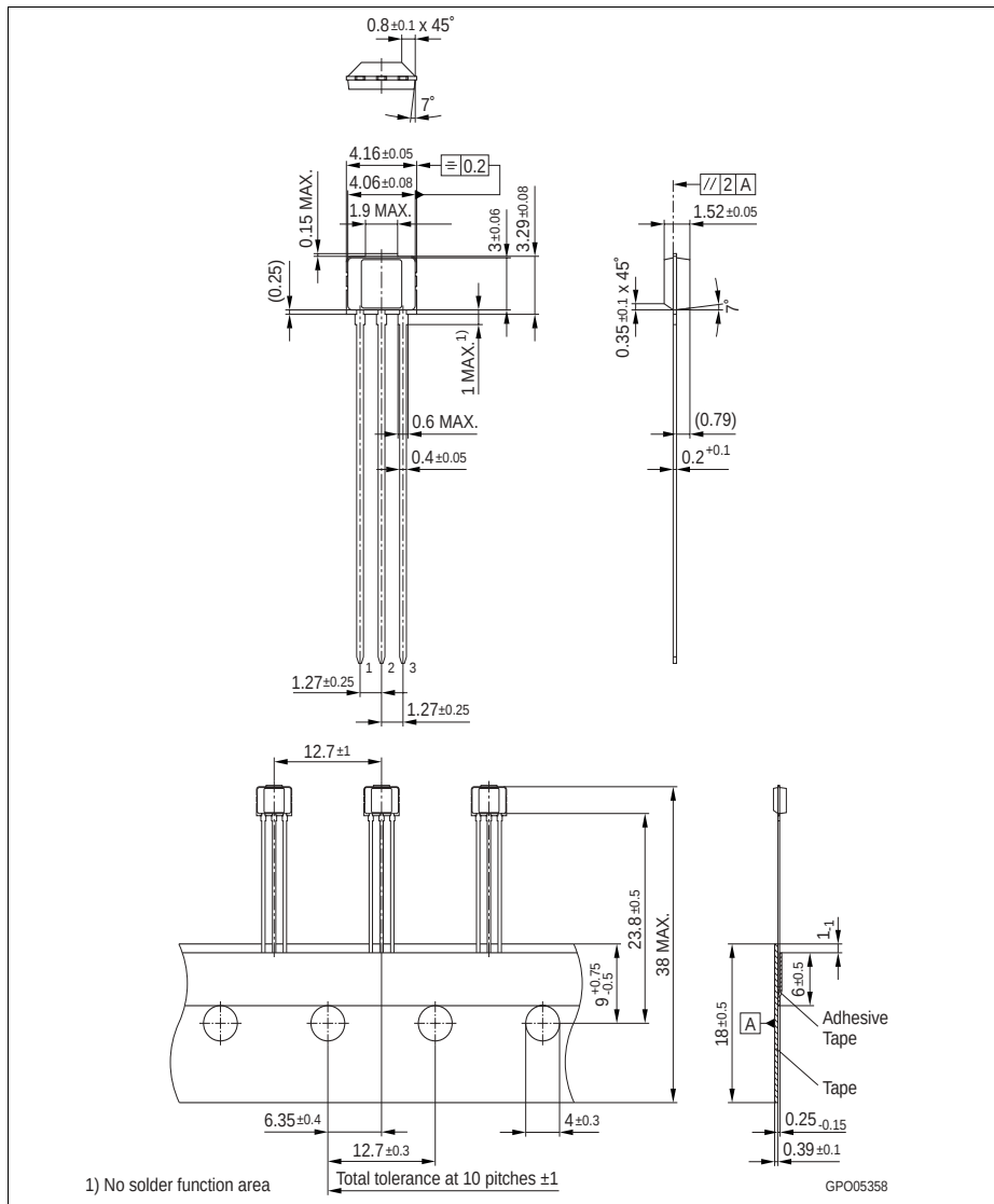
Figure 12 PG-SSO-3-2
