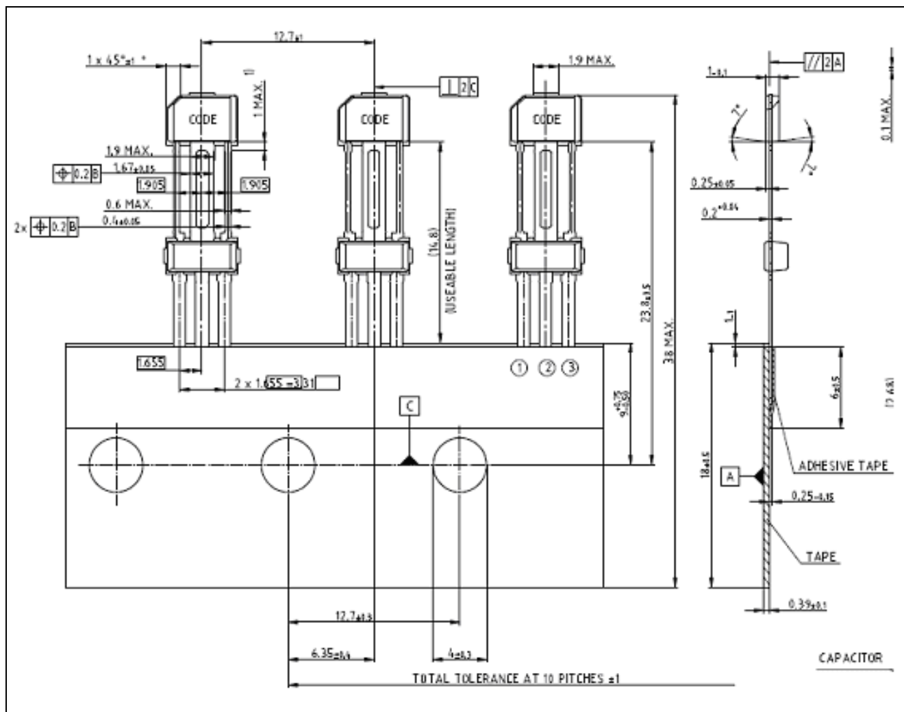
Figure 4-2 Tape loading orientation the PG-SSO-3-92
