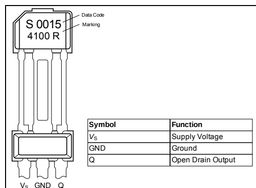
Figure 2-1 Sensor assembly
