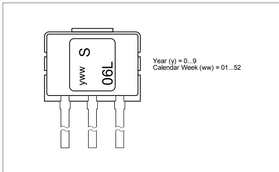
Figure 5 Marking TLE4906L
